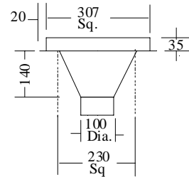
TYPE "B" SHALLOW SUMP FT7005—STANDARD FT7006—FLUSHING
