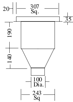
TYPE "A" EXTENDED SUMP
