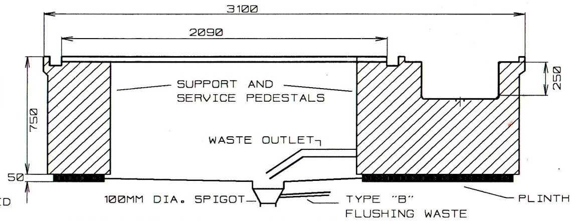
SECTIONAL ELEVATION
